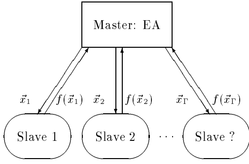
Figure 1: Master-Slave concept for the parallel evaluation of objective function values.
