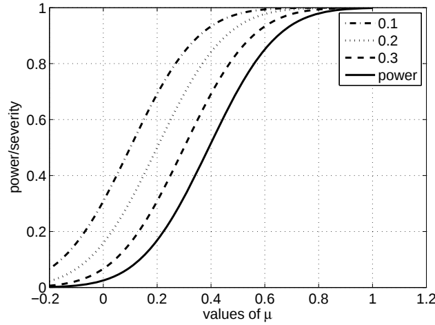
Figure 1. Case ‘Accept H_0 ’—Power versus Severity. The severity for \mu \leq 0 with different outcomes x_0 . Power curve is the solid line. Similar figure as in Mayo and Spanos (2006).
