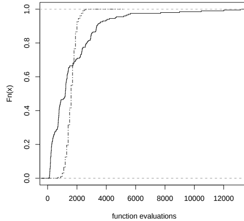
Figure 2. Run length distribution to determine an adequate number of function evaluations. The algorithm to be analyzed is run n times with different seeds on one problem instance. For each successful run, the number of function evaluations m is recorded. If the run fails, m is set to infinity. Both curves illustrate results of one algorithm on one problem instance but with different algorithm parameters. The empirical cumulative distribution shows that 2000 function evaluations are adequate, because approximately 50% of both configurations were able to reach the goal. Both parametrizations of the algorithm are able to reach the goal in nearly every run, if 10,000 function evaluations are chosen. Therefore, 10,000 function evaluations may result in ceiling effects.
