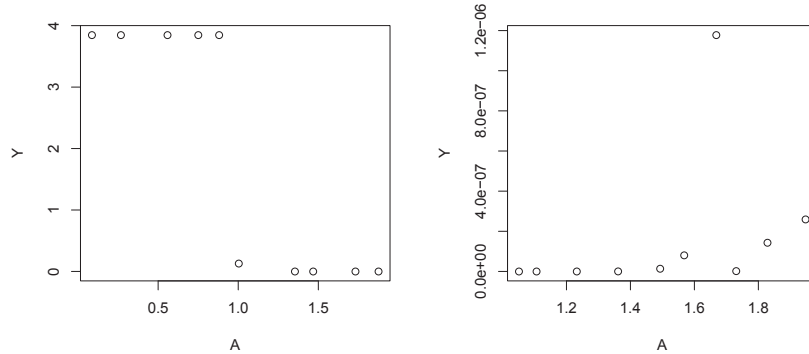
Fig. 14.3: Scatter plots from the pre-experimental planning phase to determine the region of interest. Left: A range from 0 to 2 for the multiplier a was chosen. Values smaller than 1 invert the 1/5th rule (2.4). As can be seen from the figures, values smaller than 1 worsen the performance of the (1+1)-ES. Right: If a is chosen from the interval between 1 and 2, the (1+1)-ES performs quite reasonably. These results support the recommendations given in (2.4)
