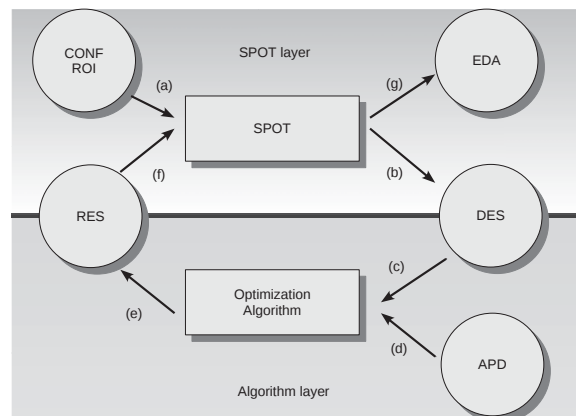
Fig. 14.1: SPOT interfaces. The SPOT loop can be described as follows: Configuration (CONF) and region-of-interest (ROI) files are read by SPOT (a). SPOT generates a design (DES) file (b). The algorithm reads the design file and (c) extra information, e.g., about the problem dimension from the algorithm-problem design (APD) file (d). Output from the optimization algorithm are written to the result (RES) file (e). The result file is used by SPOT to build the prediction model (f). Data can be used by exploratory data analysis (EDA) tools to generate reports, statistics, visualizations, etc. (g)
