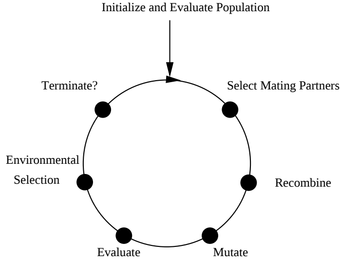
Fig. 1. Evolutionary algorithms.
