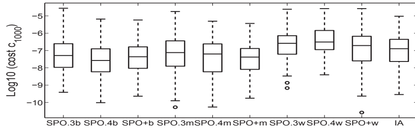
(a) CMAES-Sphere
