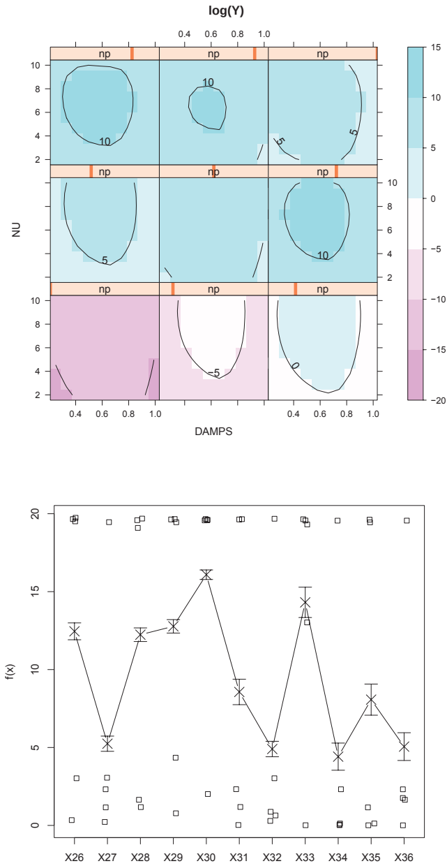
Fig. 15.17: Top : Contour plot based on the complete data set (CMAES-Sphere, 49 data points). Smaller values are better. The factor which has the smallest effect, CS, is held constant. NU is plotted versus DAMPS, while values of the factor with the last but one effect, namely NPARENTS (np), are varied with the slider on top of each panel. Bottom : Function values f(x) (Ackley) versus steps along the path of the steepest descent. Indices denote the eleven steps from the steepest descent. Note that these values are based on five repeats
