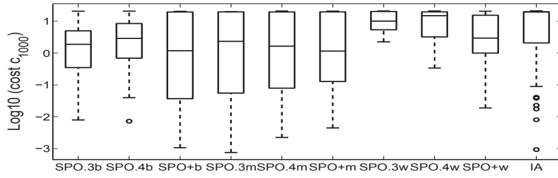
(b) CMAES-Ackley
