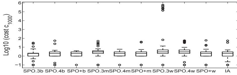
(c) CMAES-Rastrigin
