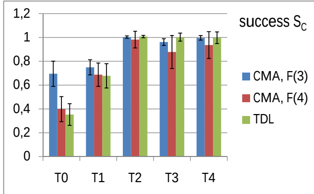
Figure 2: Success S_C acc. to Eq. (8) for the different algorithms CMA[ F^{(3)} ], CMA[ F^{(4)} ] and TDL (from left to right in each group) as a function of the feature sets. Each bar represents the average of 25 realizations based on G = 60000 games of training using the feature set as indicated on the horizontal axis. Error bars indicate one standard deviation
