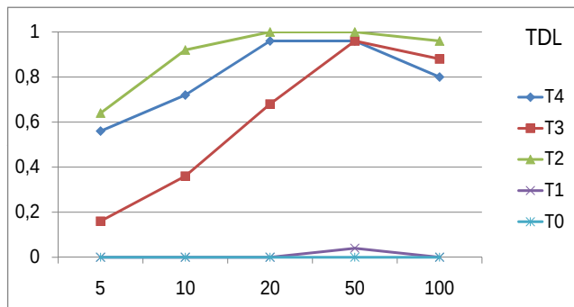
Figure 4: Comparison of different feature sets: Same as Fig. 3 but with TDL instead of CMA-ES.
