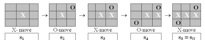
Figure 1: Some after states for the game TicTacToe
