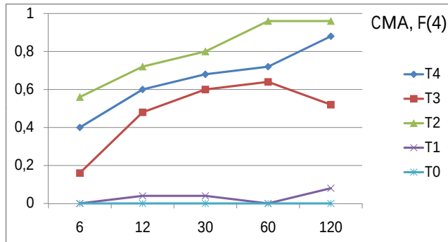
Figure 3: Comparison of different feature sets: Shown is the success rate p_S (percentage of successful players out of 25 realizations, acc. to Eq. (7)) as a function of the number of games G divided by 1000. All results were obtained with CMA-ES used for neuroevolution of a feedforward net having one hidden layer with 15 neurons. The upper diagram uses fitness function F^{(3)} and the lower uses fitness F^{(4)} with R = 4 and n^{(Pool)} = 3 .
