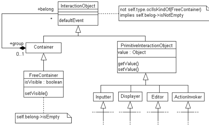
Fig. 3. The Abstract Presentation Pattern
