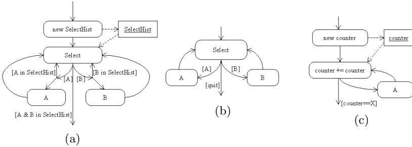
Fig. 7. The UML modelling of three common interaction application behaviours. An order independent behaviour is modelled in (a). An optional behaviour is modelled in (b). A repeatable behaviour is modelled in (c).
