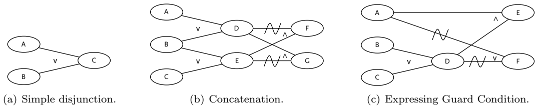
Figure 2: Cause-effect graphs.
